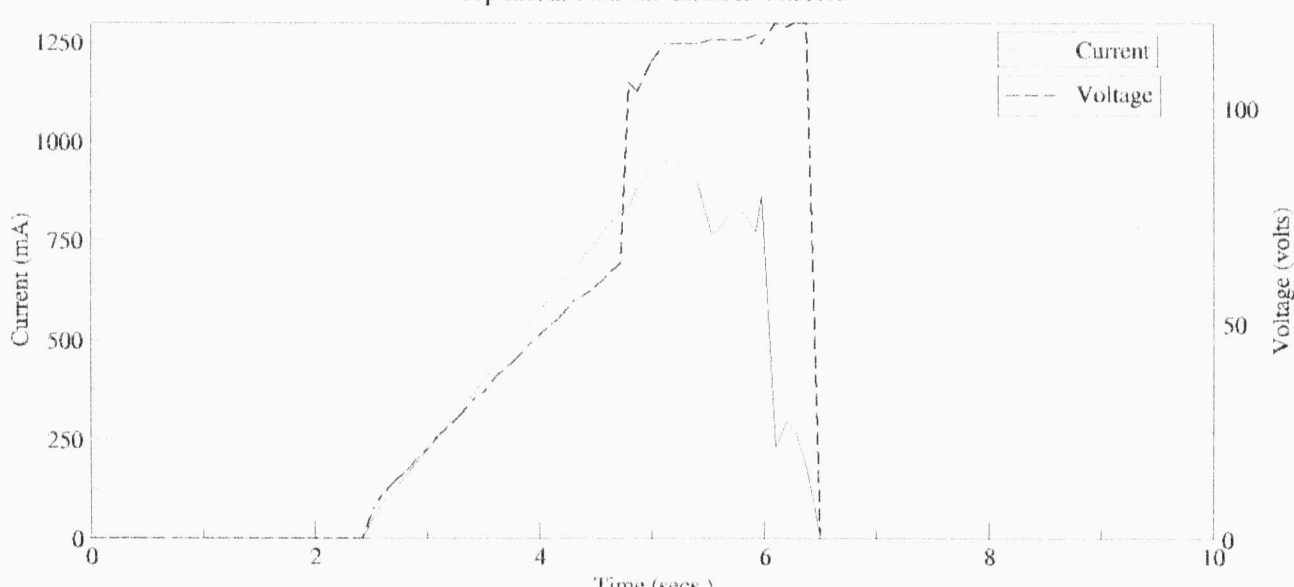
Shot V-I Characteristics Top shot at 149.94m 02/22/09 14:33:12
