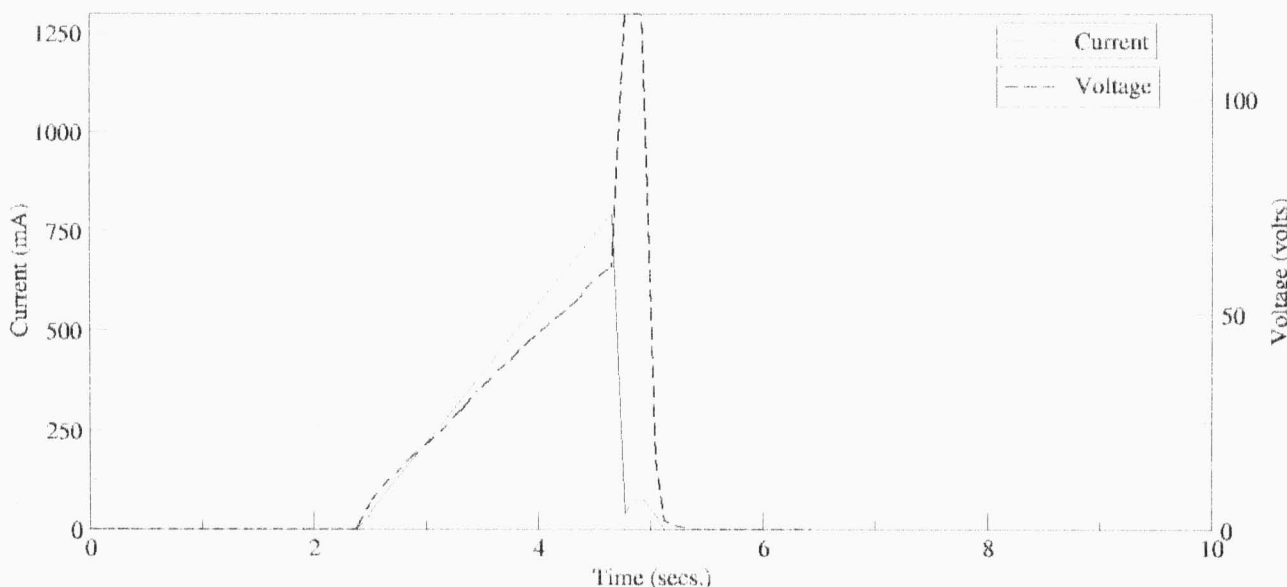
Shot V-I Characteristics Top shot at 150.00m 02/23/09 12:09:28
