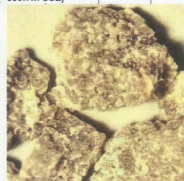
Slave Point Limestone 20X 1371m - 1377m
