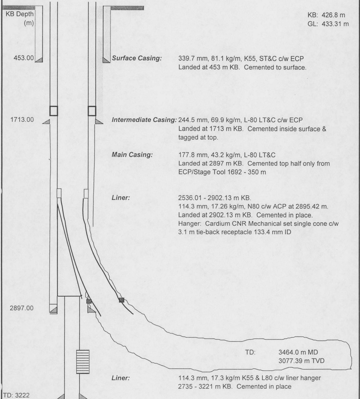
Diagram I (Actual as of March, 1999) See Diagram II for Tubing Details
