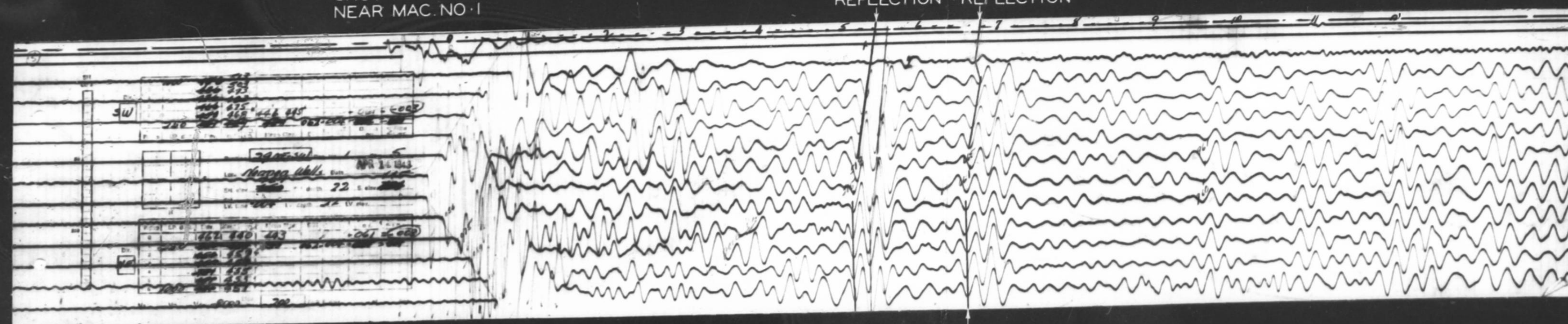
SHOT POINT 29 3 1/2 MILES S.W. OF MAC NO. 1
