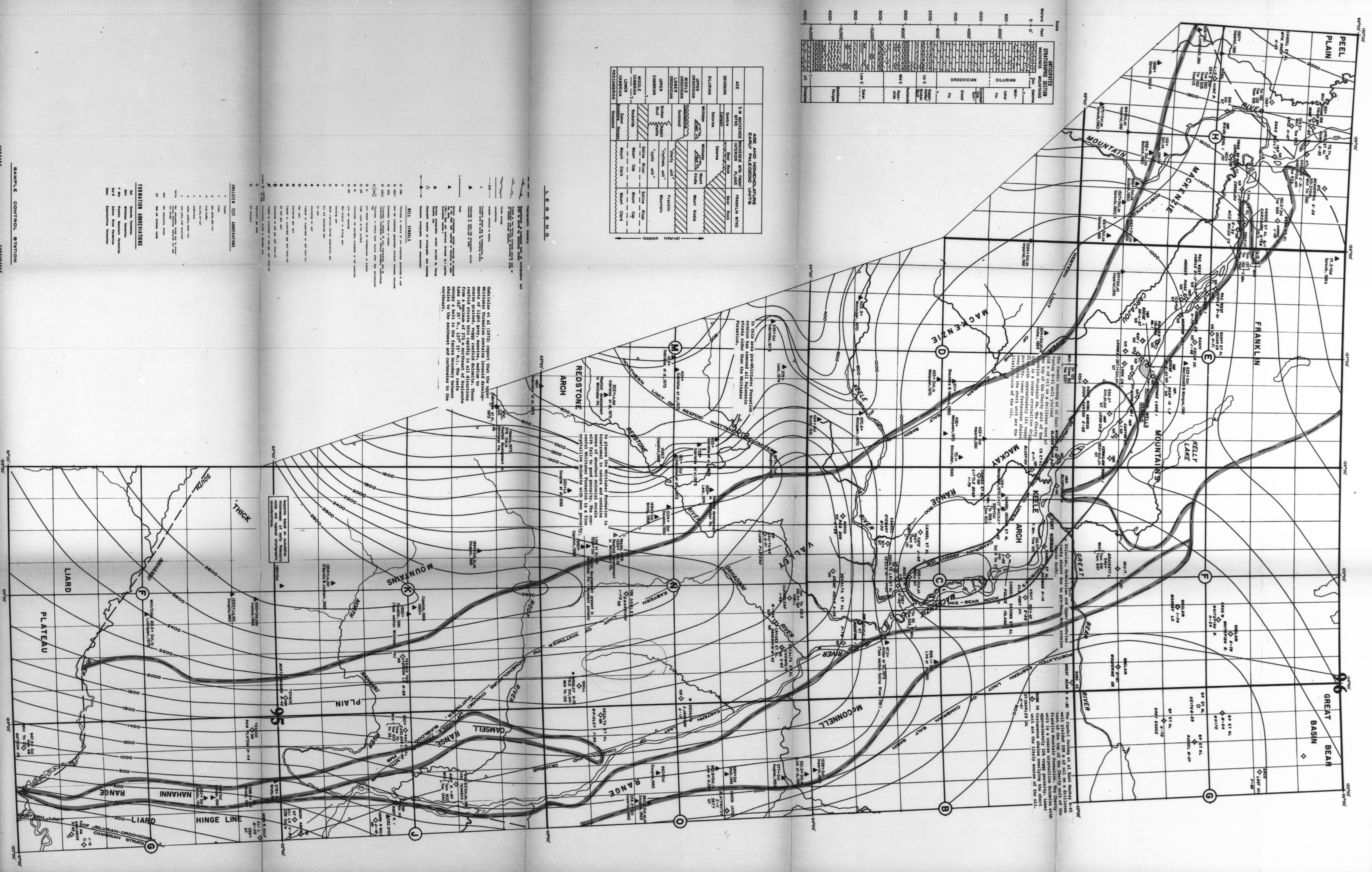
STRATIGRAPHIC MAP OF THE SILURIAN, OROVIAN AND CAMBRIAN IN THE MACKENZIE VALLEY PLAIN MACKENZIE BASIN AREA
