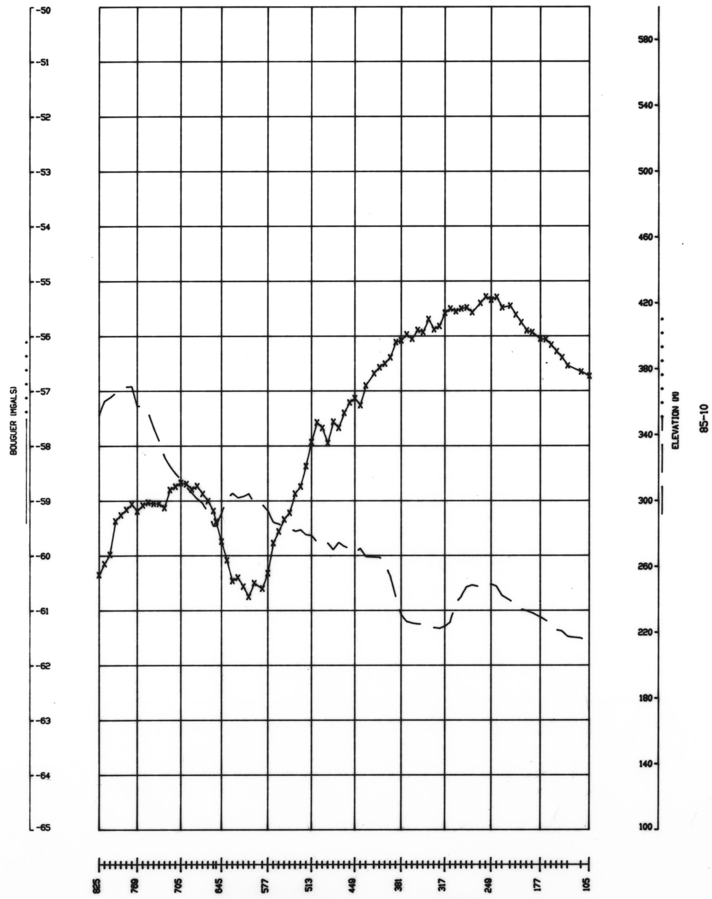
BOUGUER AND ELEVATION PROFILE - LINE 85-10
