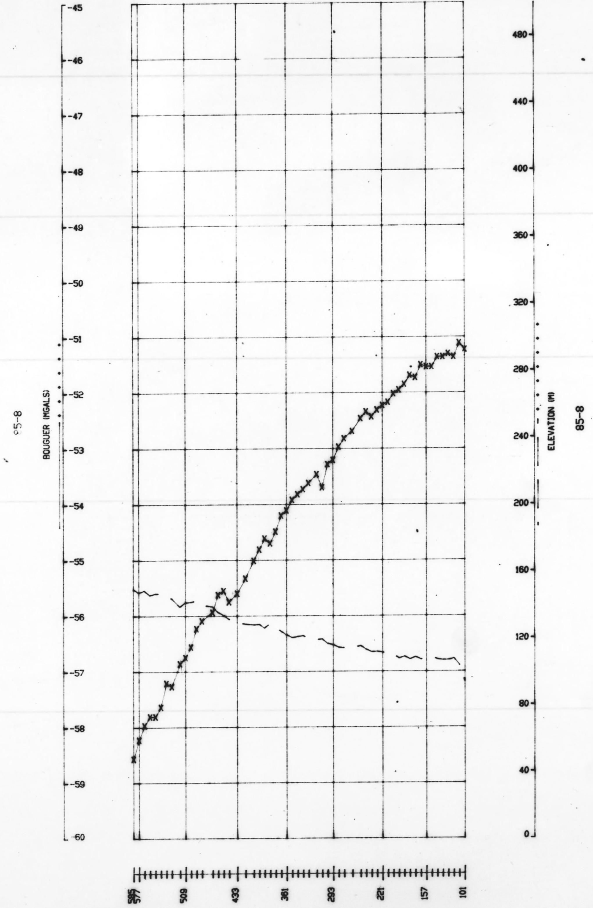
BOUGUER AND ELEVATION PROFILE - LINE 85-8
