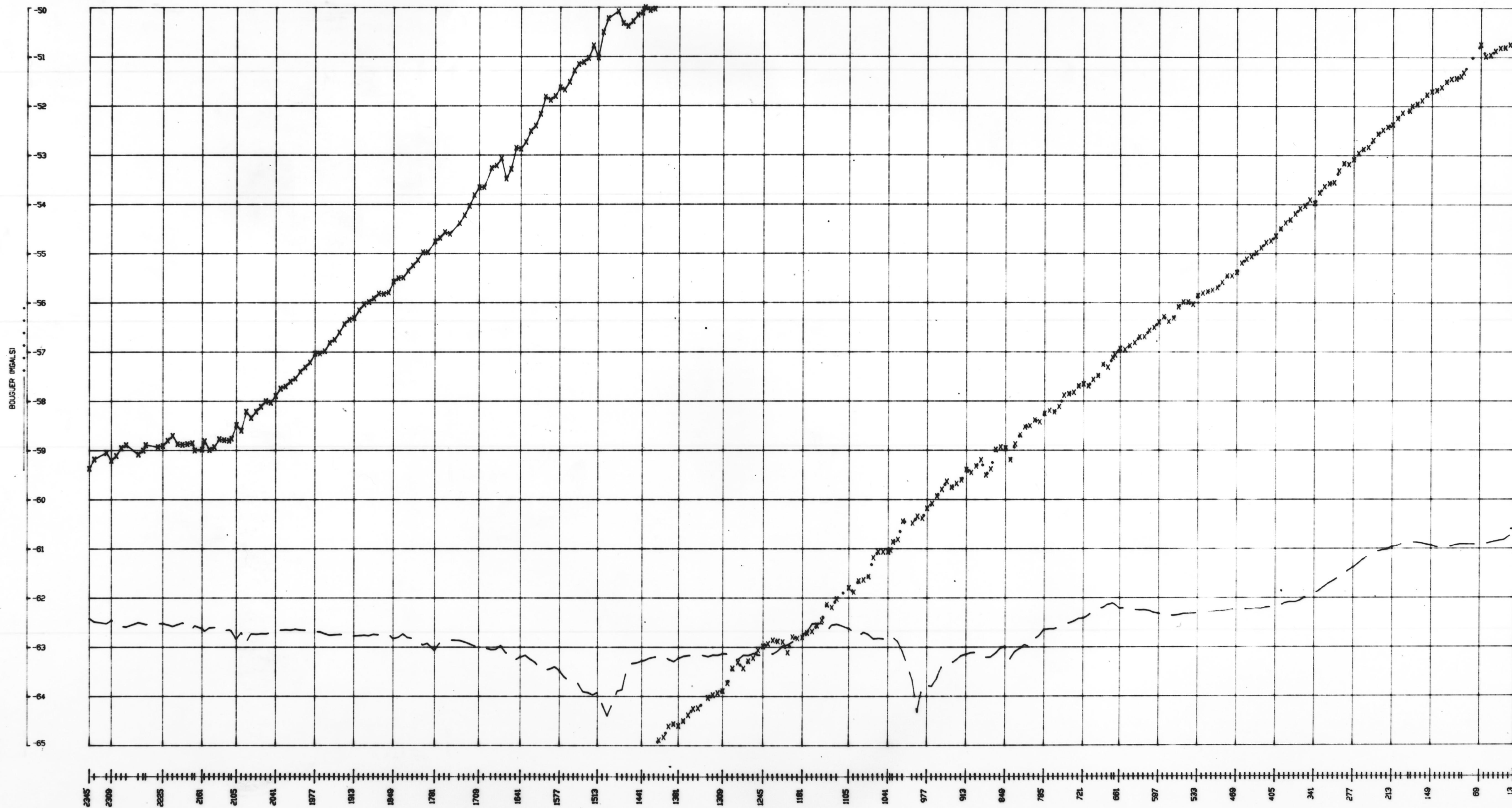
BOUGUER AND ELEVATION PROFILE - LINE 85-7B
