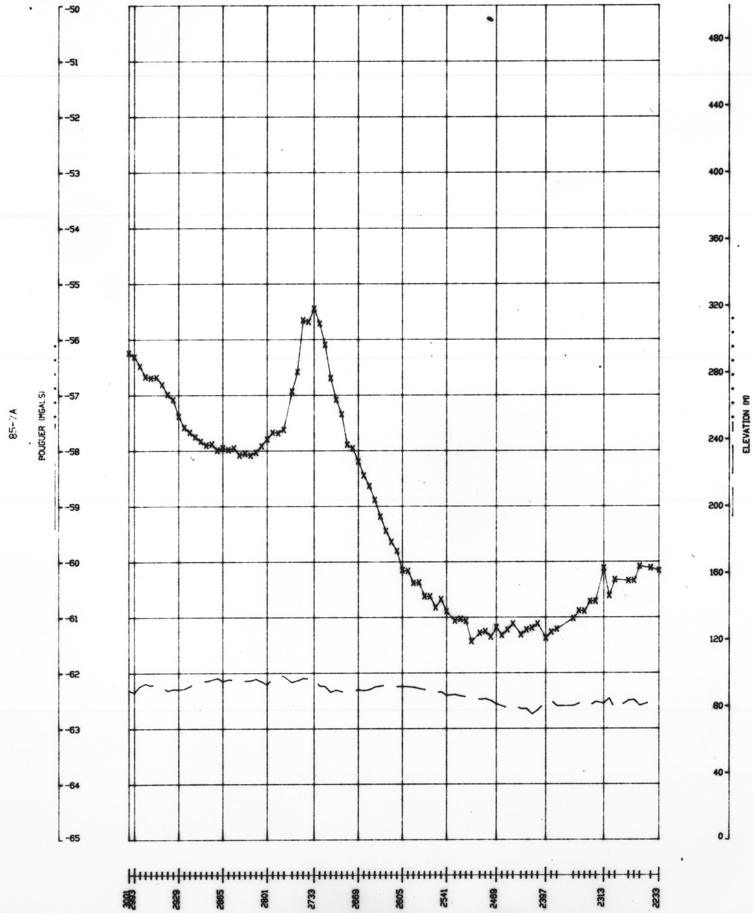
BOUGUER AND ELEVATION PROFILE - LINE 85-7A
