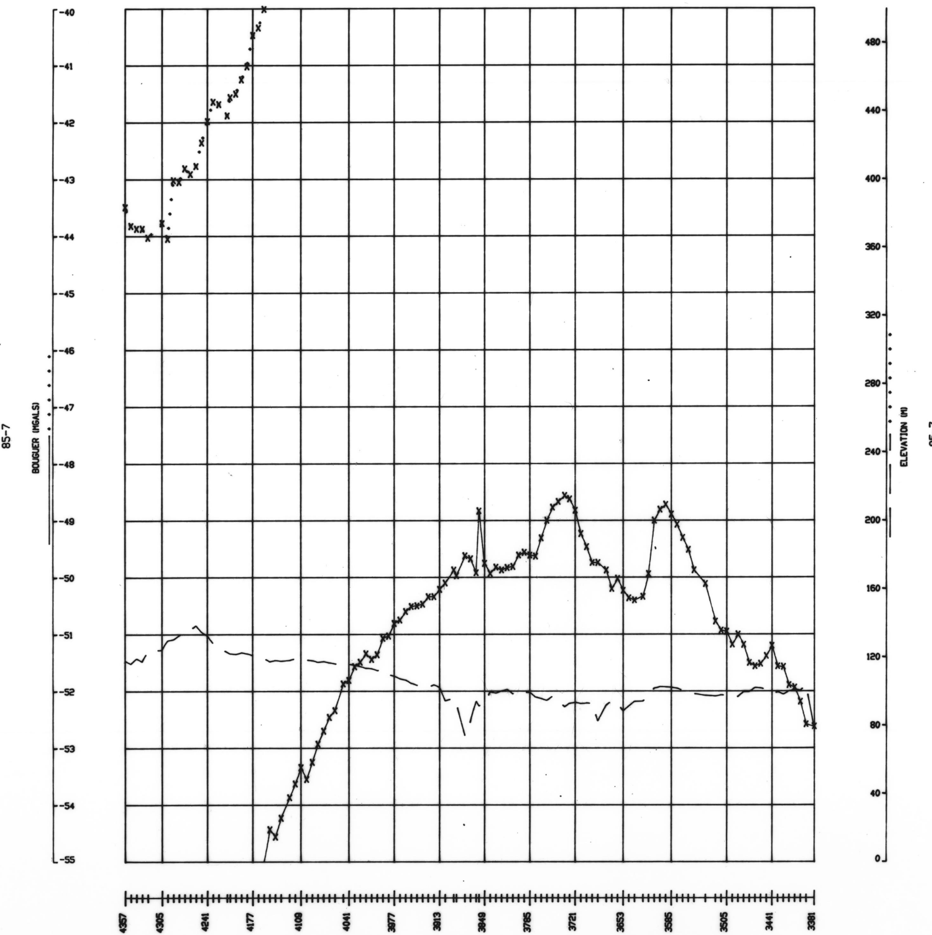
BOUGUER AND ELEVATION PROFILE - LINE 85-7
