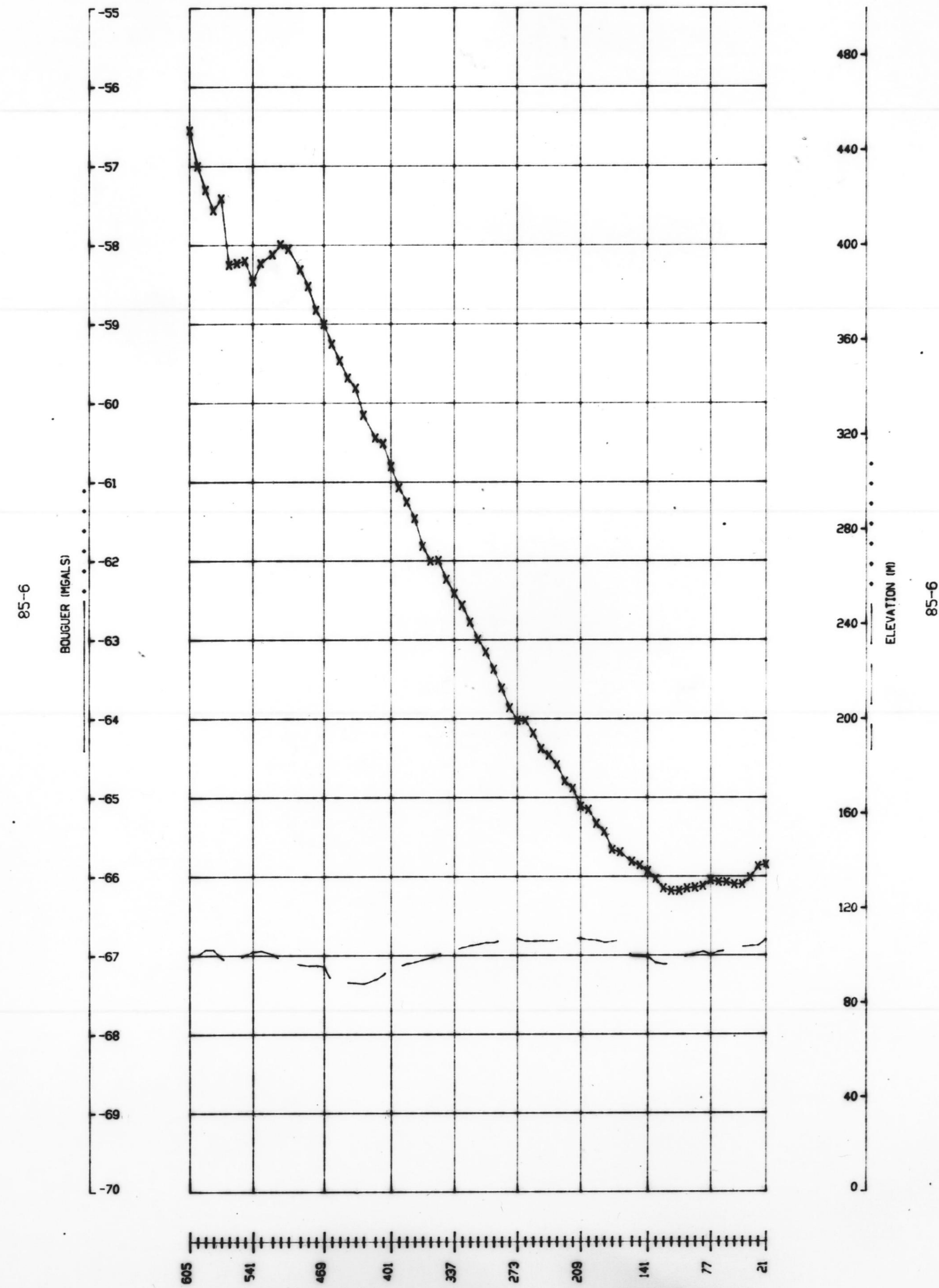
BOUGUER AND ELEVATION PROFILE - LINE 85-6
