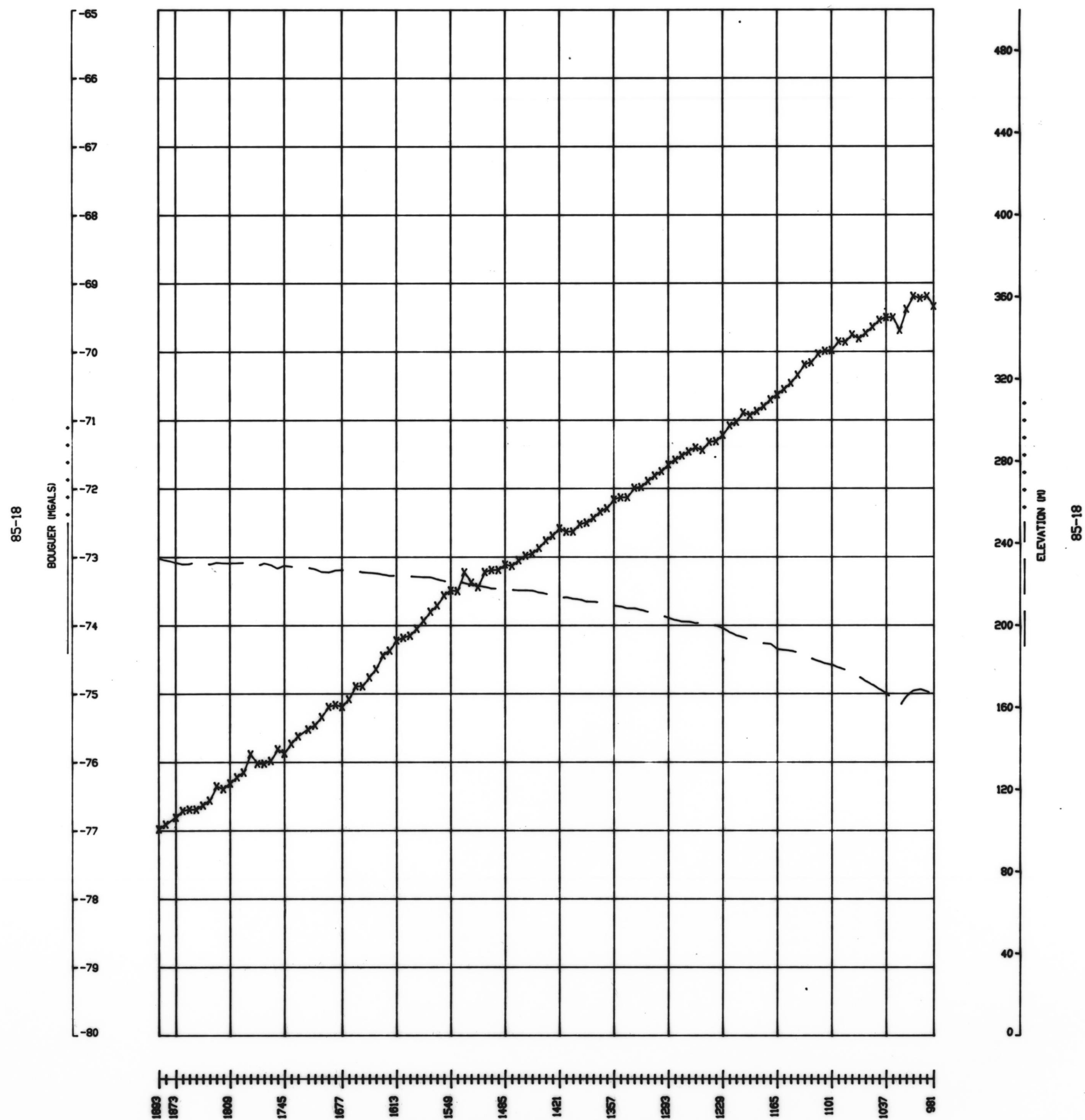
BOUGUER AND ELEVATION PROFILE - LINE 85-18
