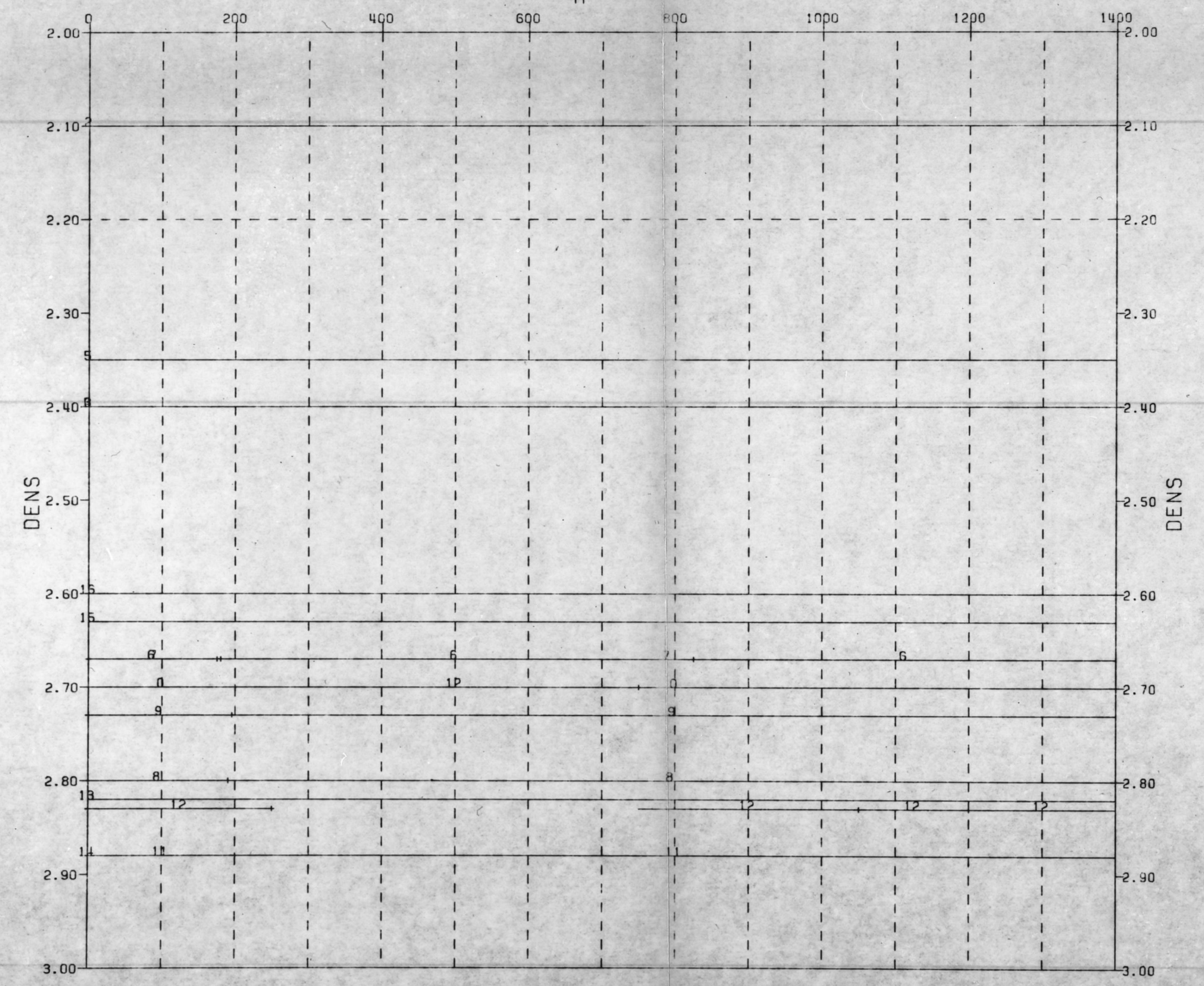
DENSITY MODEL - CARBONATE BUILDUP KHMODEL3 UPPER KEG CARBONATE BUI
