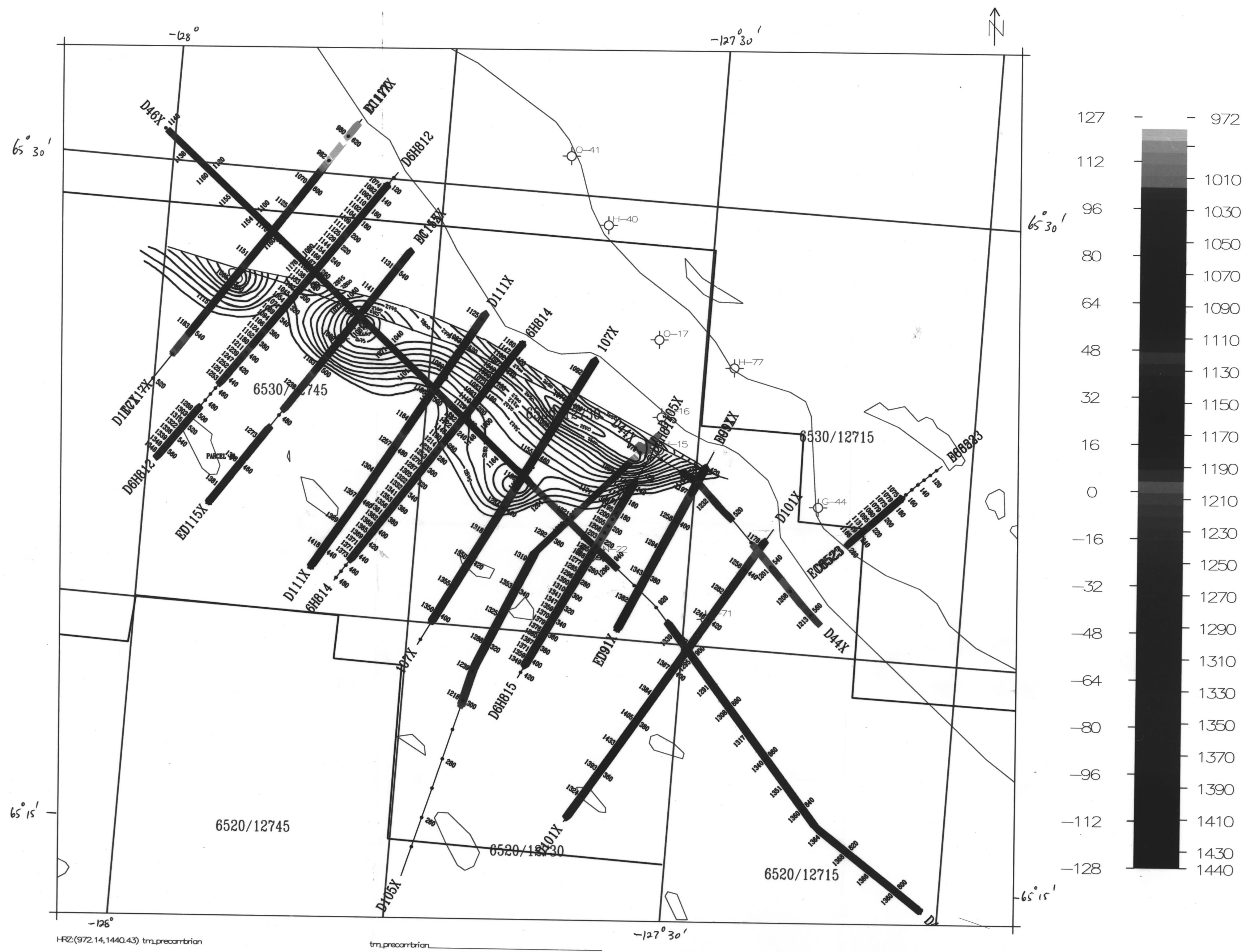
9227-E35-1E EL401 - Precambrian Structure Map (from pre-stack depth migrated seismic) 0m 5000m 10000m 1cm = 1000 meters
