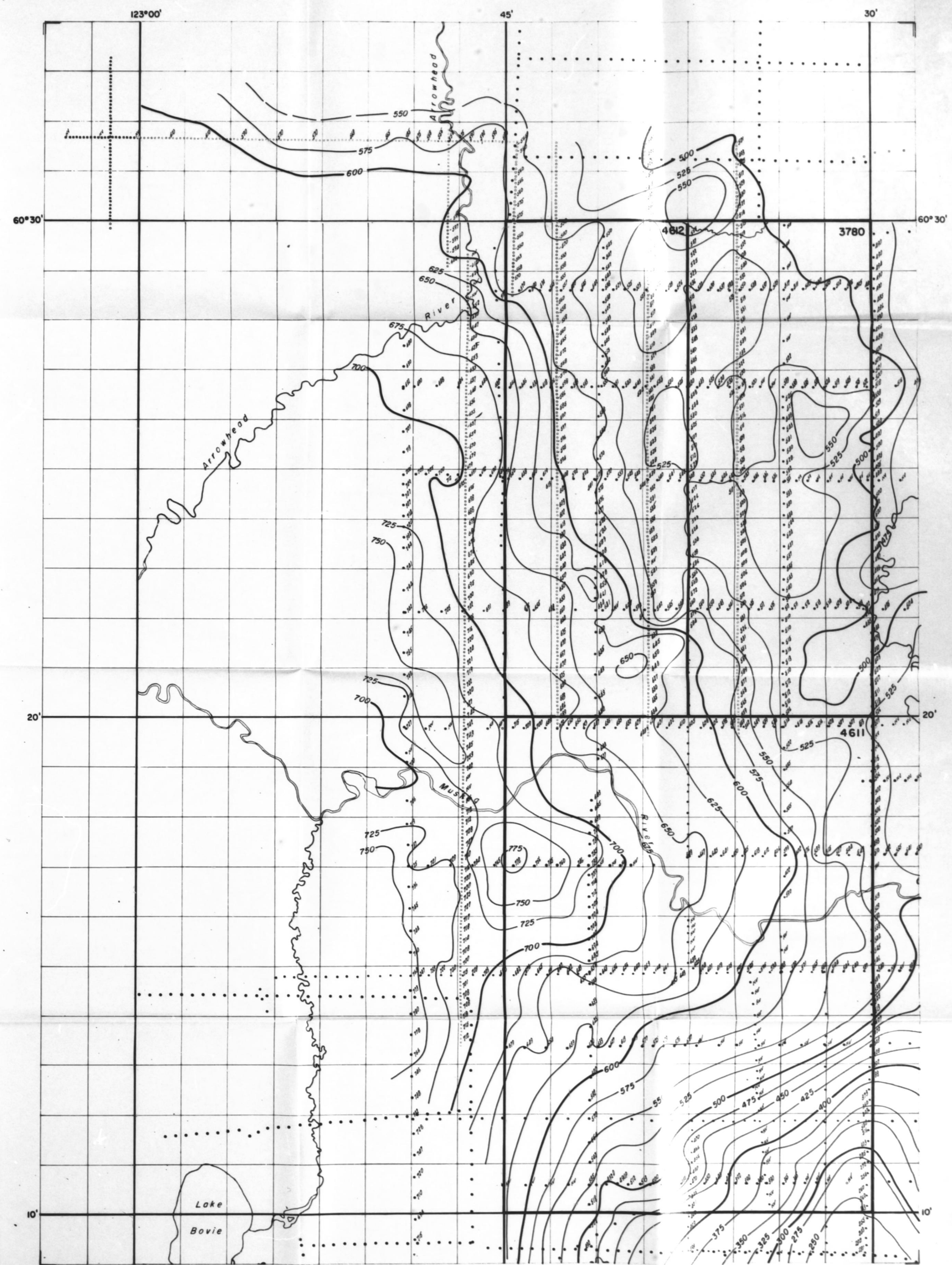
P. & N. G. PERMITS 3780, 4611 & 4612 TIME STRUCTURE ON BANFF FORMATION CONTOUR INTERVAL - 25 MILLISECONDS DATUM ELEV. +1500' DATUM VELOCITY 9000'/SEC.
