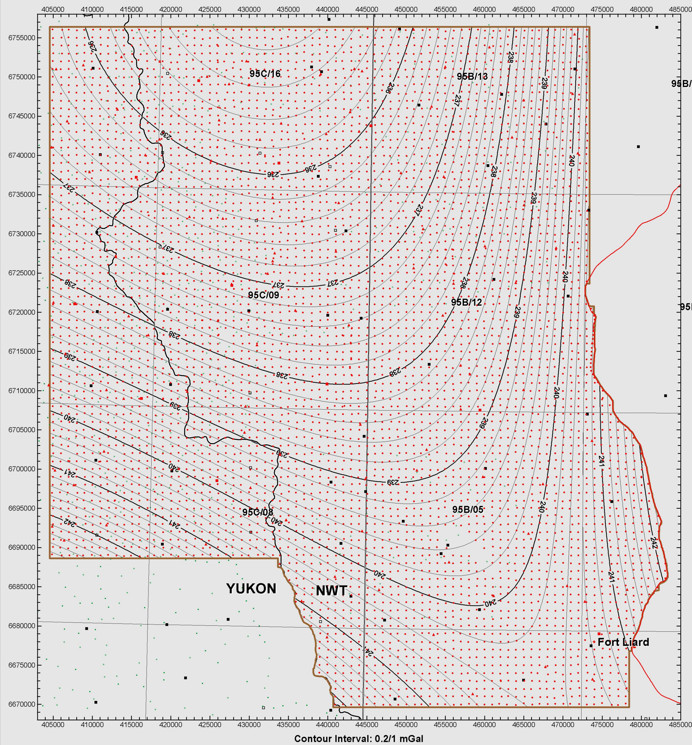
Regional Gravity - Polynomial Filter
