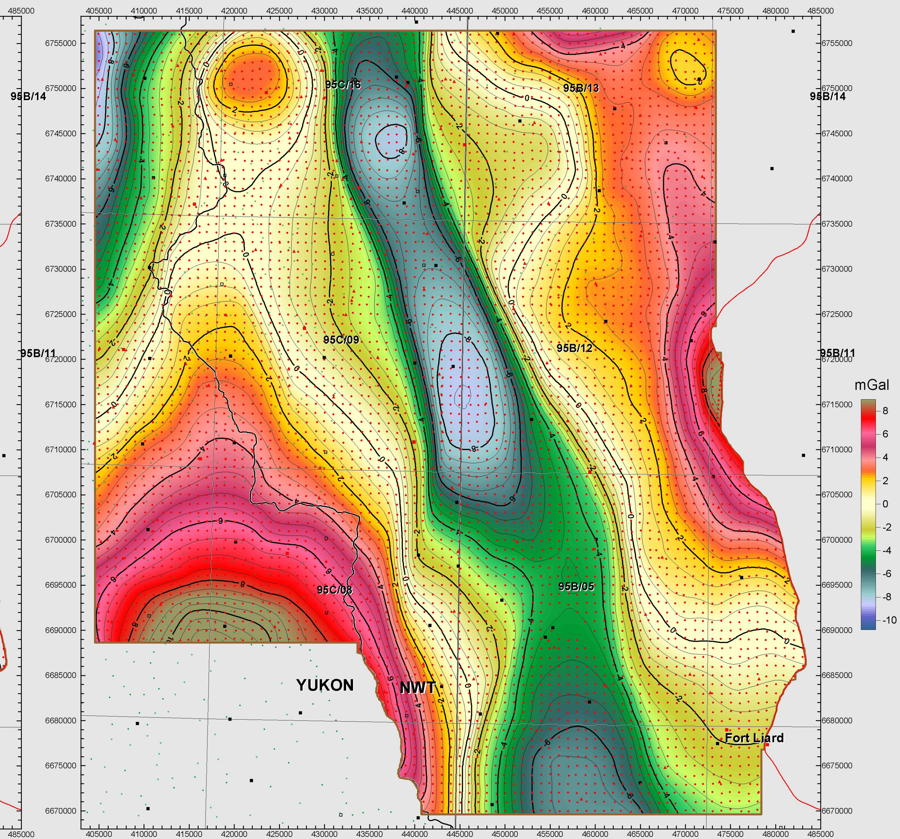
Regional Gravity - 8 km Filter
